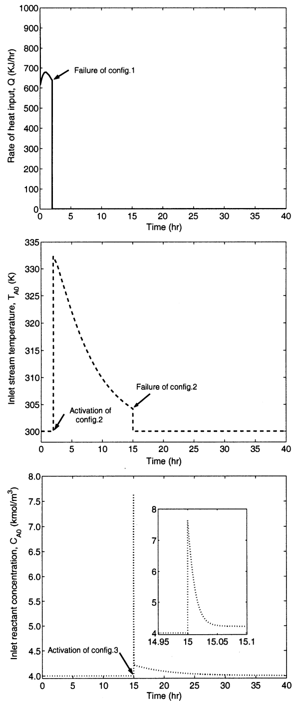
Figure 15. Manipulated input profiles under the Q -control configuration (top), the T_{A0} -control configuration (middle), and the C_{A0} -control configuration: T_{A0} starts to vary only after the first configuration fails at t = 2.0 h, while C_{A0} begins to vary after the second configuration fails at t = 15 h.
