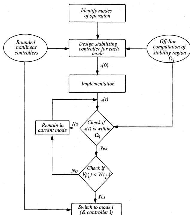
Figure 5. Hybrid control strategy based on coordinating feedback and switching.
