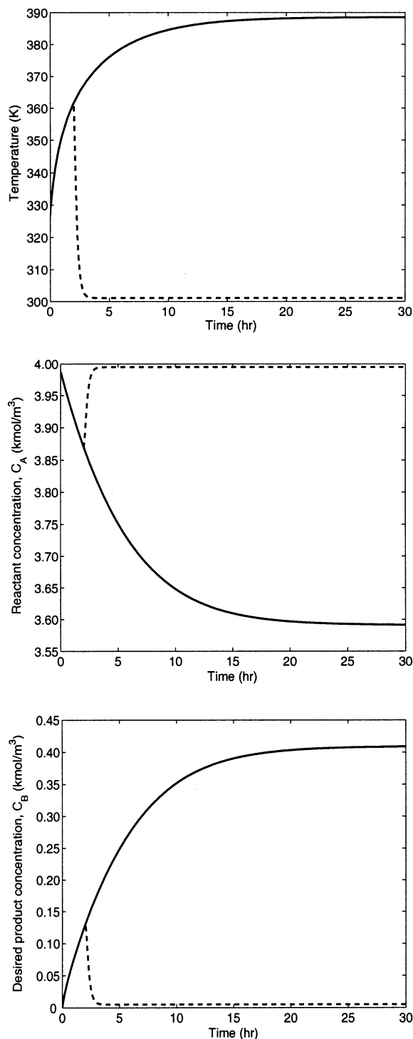
Figure 12. Evolution of the closed-loop temperature (top), reactant concentration (middle), and desired product concentration (bottom) profiles when the primary control configuration operates without failures (solid profiles), and when it fails at t = 2.0 h (dashed profiles) without activating any of the backup control configurations.
